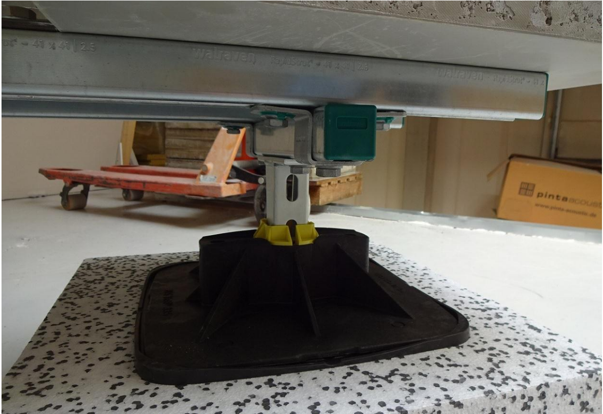
Photo 9: Measurement 7, detail BIS Yeti® Support System, type 335, placed on EPS-insulation
