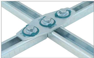
X connector in use with RapidRail®
