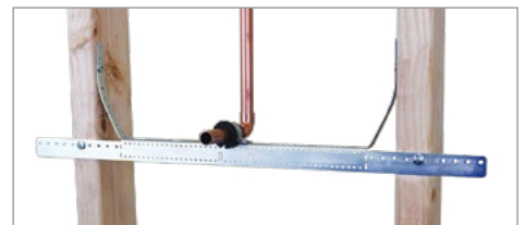
Heavy Angled Wall Bracket in use with single CPVC/copper stub-out clamp.
