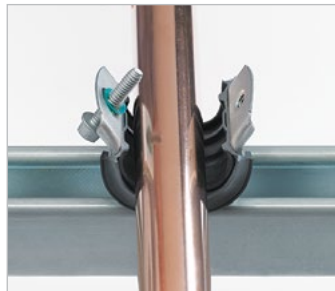
2. Insert pipe
