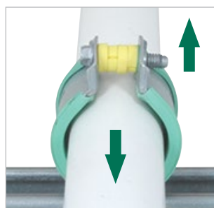
Use spacers for sliding points
