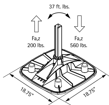
Adjustable to compensate roof pitch up to 7°
