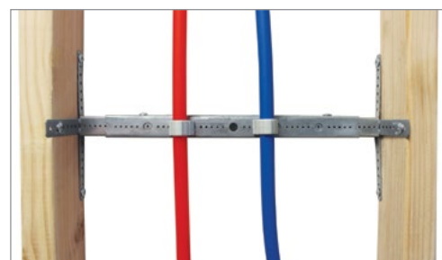
Multi-Purpose Telescoping Support in use with starQuick® clamps
