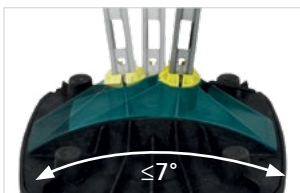
Adjustable to compensate roof pitch up to 7°
