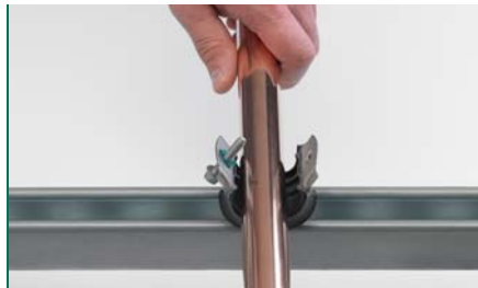
2 Insert pipe
