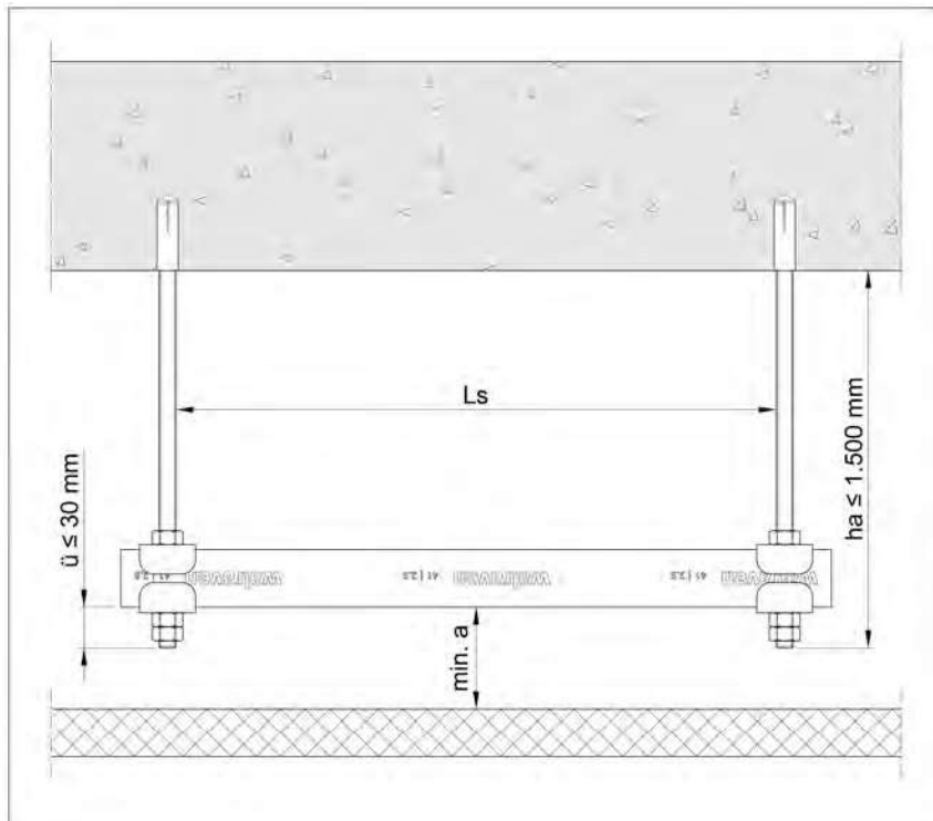
Figure 1: Example of a mounting rail in the ceiling plenum of suspended ceiling construction in accordance with the Specimen Conduit Guideline [German designation: MLAR], edition of 10/02/2015, Section 3.5.3.
