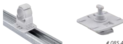
starQuick® Universeel Rail Adapter
