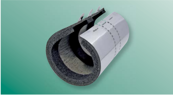
BIS Pacifyre® MK II Fire Sleeve Single component built-in fire sleeve for fire safe and smoke tight sealing of pipe apertures.
